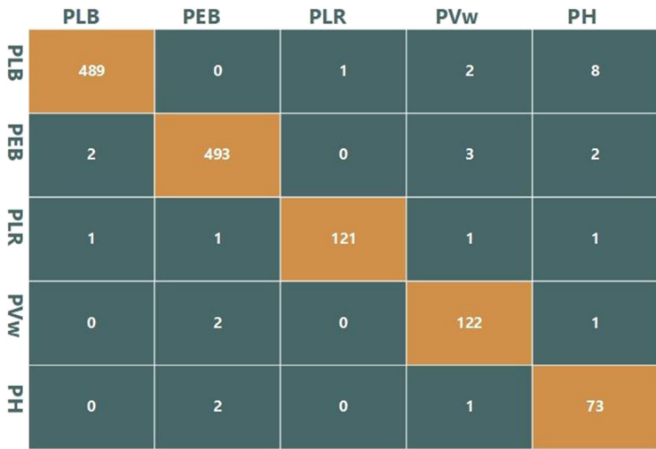
Figure 5. Confusion matrix for the proposed classifier.
